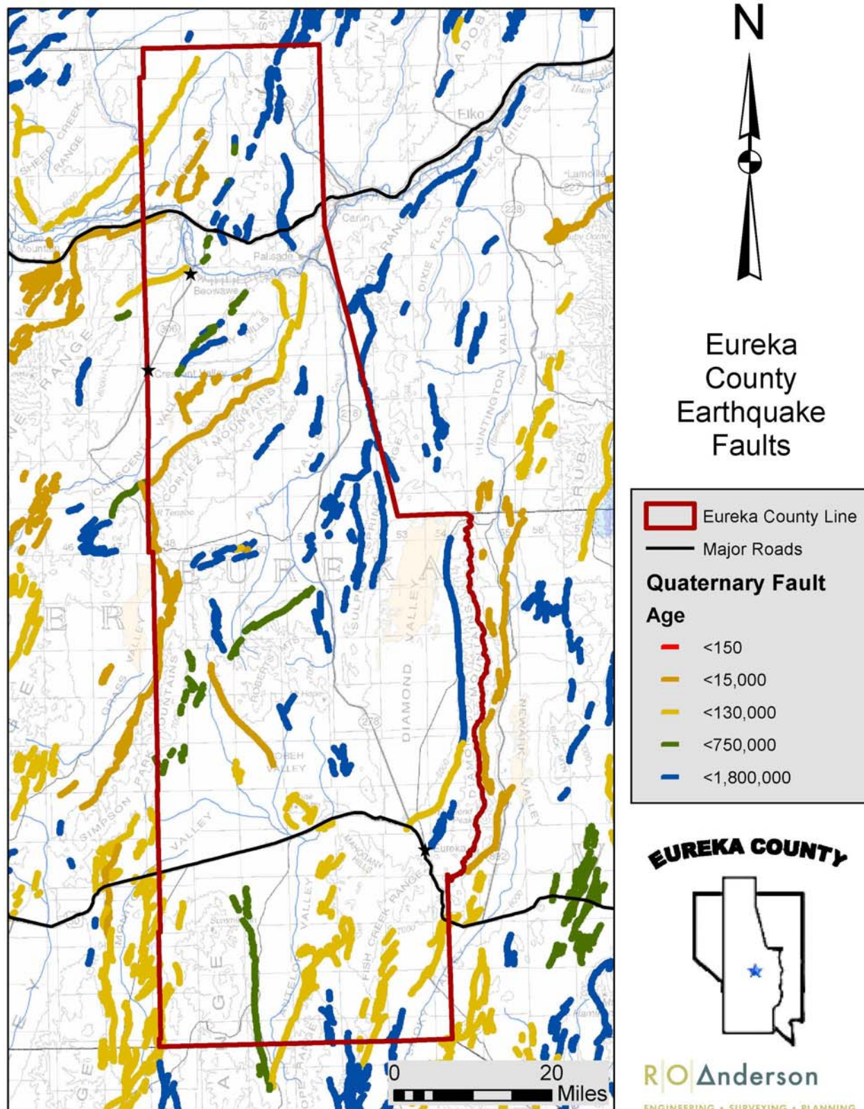
Figure B-3: Eureka County Earthquake Faults
