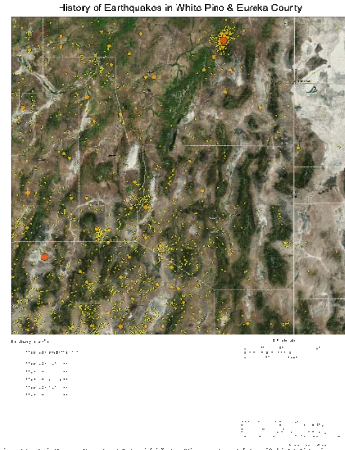
Figure 5-2: Historic Earthquakes in Nevada
